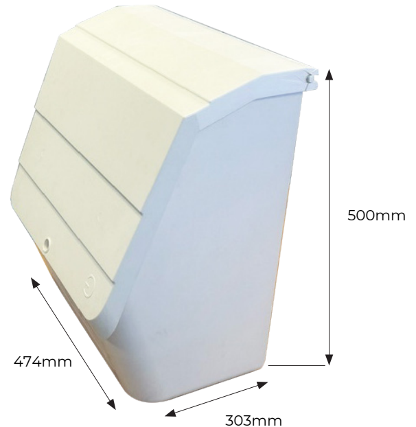
Example: Universal Smart Gas Meter Box
